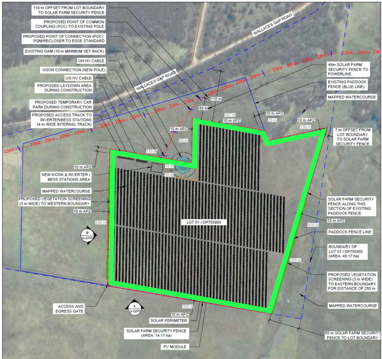
Figure 3 – Majors Creek 1A Solar Farm & BESS project General Arrangement with the APZ in highlight
